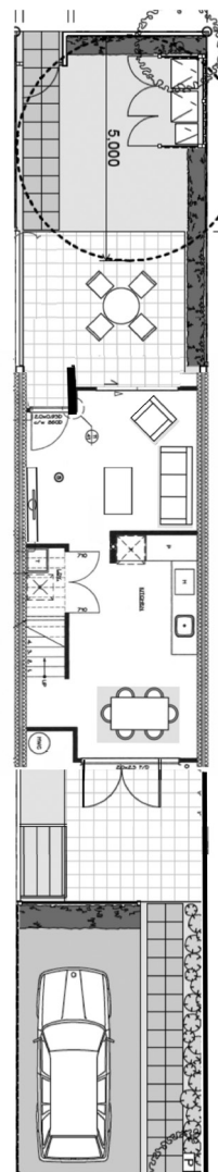
Ground Floor
